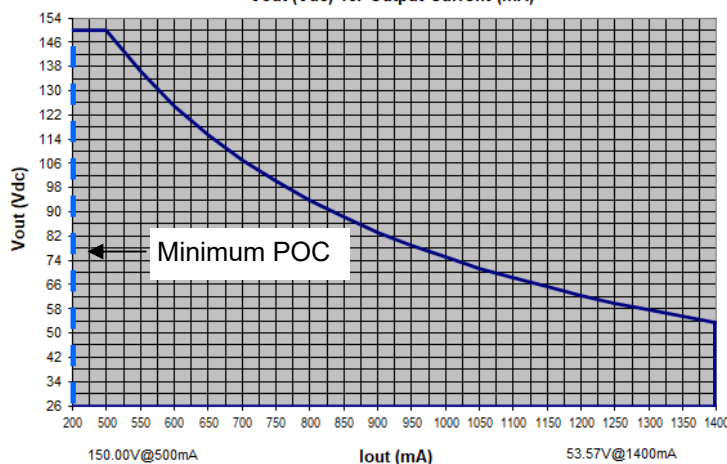
LPF75W-150-PC1400-RD OPERATING WINDOW Vout (Vdc) vs. Output Current (mA)
