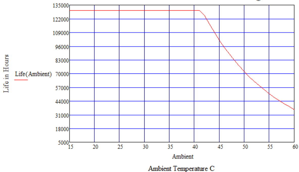
LPF75W-XX-PCXXXX-RD Estimated Life Full Load @ 120Vac
