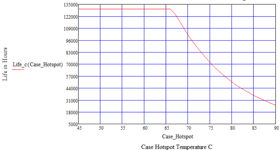
LPF75W-XX-PCXXXX-RD Estimated Life Full Load @ 120Vac
