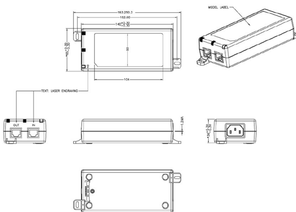
PoE Injector (98-9000311-01)
