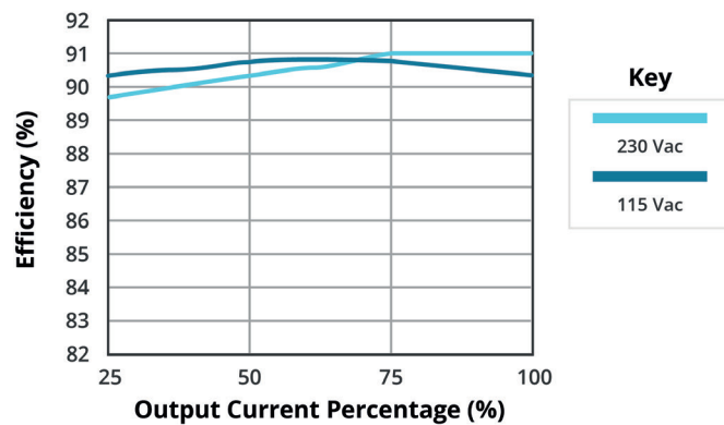
EFFICIENCY VS OUTPUT LOAD VOF-85B-48 (natural convection)
