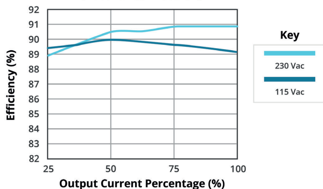
EFFICIENCY VS OUTPUT LOAD VOF-85B-12 (natural convection)
