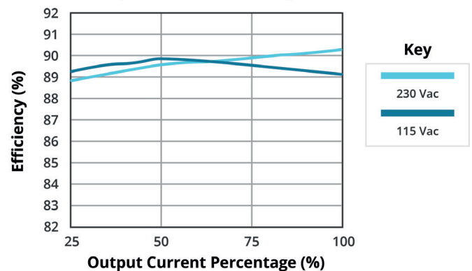
EFFICIENCY VS OUTPUT LOAD VOF-85B-24 (natural convection)
