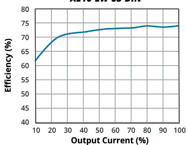
EFFICIENCY VS OUTPUT LOAD AE10-EW-S5-DIN
