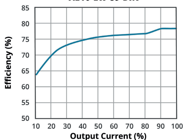
EFFICIENCY VS OUTPUT LOAD AE10-EW-S9-DIN
