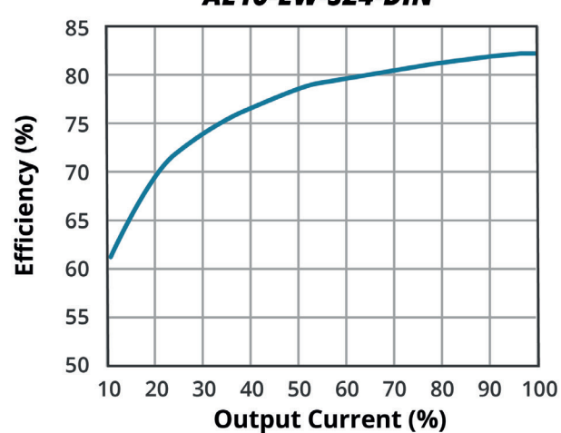
EFFICIENCY VS OUTPUT LOAD AE10-EW-S24-DIN
