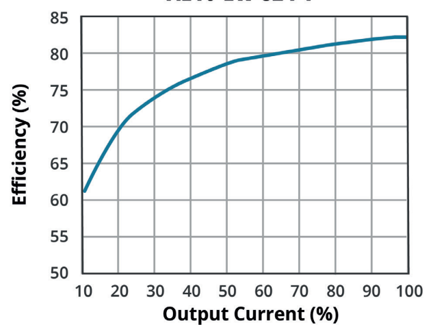
EFFICIENCY VS OUTPUT LOAD AE10-EW-S24-T
