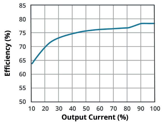
EFFICIENCY VS OUTPUT LOAD AE10-EW-S9-T
