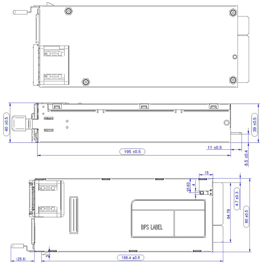
Figure 22.1. Top, bottom and side view
