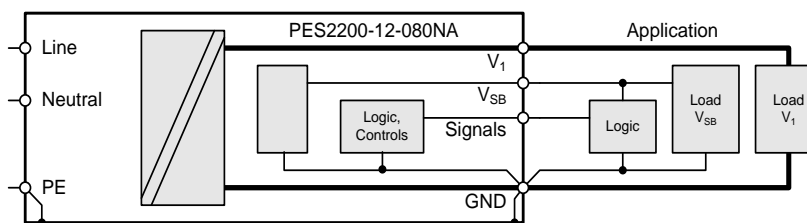
Figure 6. Separated Power and Signal Ground
