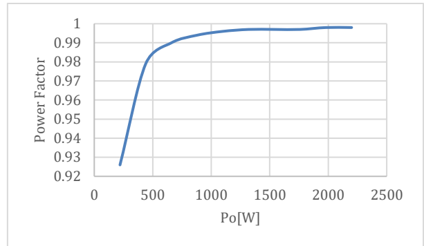
Figure 3. Power factor vs. Load
