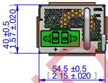
Figure 3. Front View
