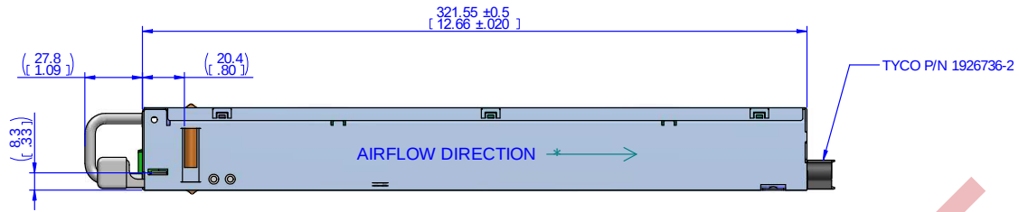
Figure 1. Side View 1
