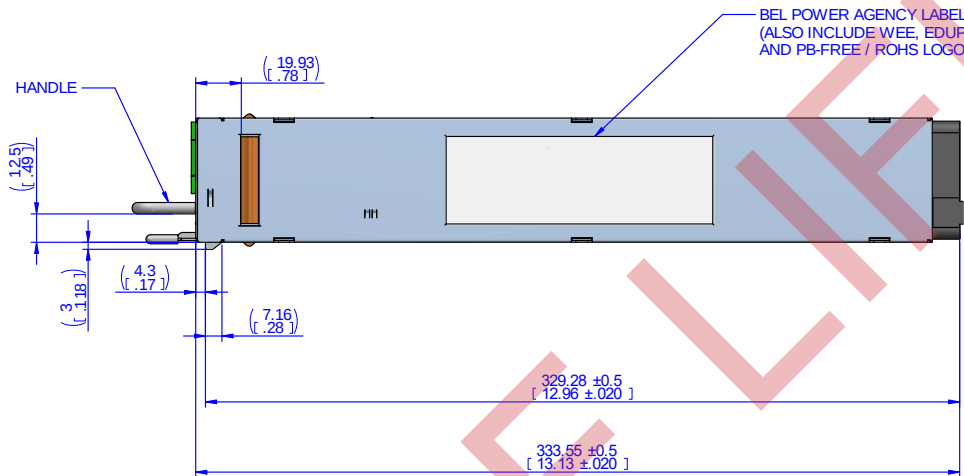
Figure 2. Top View
