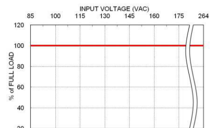
MAD40 Derating Curve vs. Input Voltage
