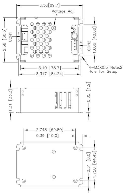
BOTTOM VIEW
