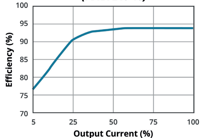
EFFICIENCY VS OUTPUT LOAD (PDRA-240-48)
