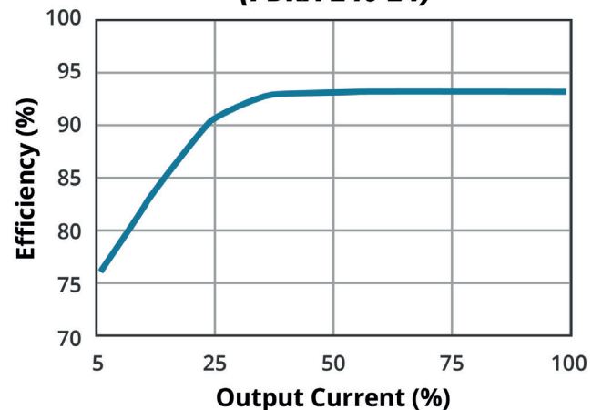
EFFICIENCY VS OUTPUT LOAD (PDRA-240-24)
