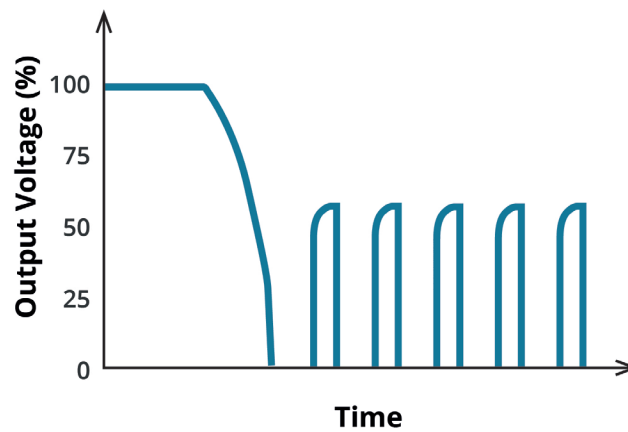
OUTPUT VOLTAGE VS TIME HICCUP MODE
