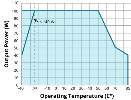
TEMPERATURE DERATING CURVE 5 Vdc output model
