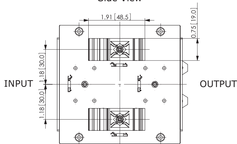
Bottom View
