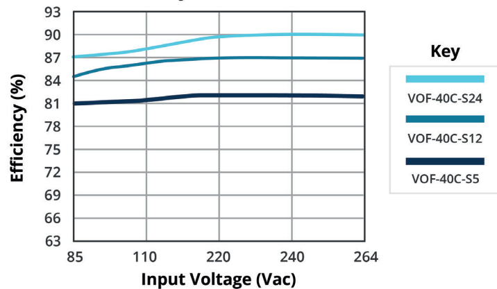
EFFICIENCY VS INPUT LOAD (full load)
