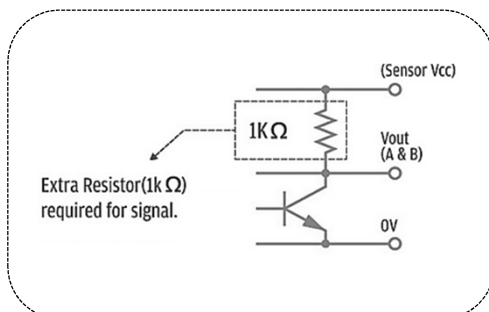
Output Circuit
