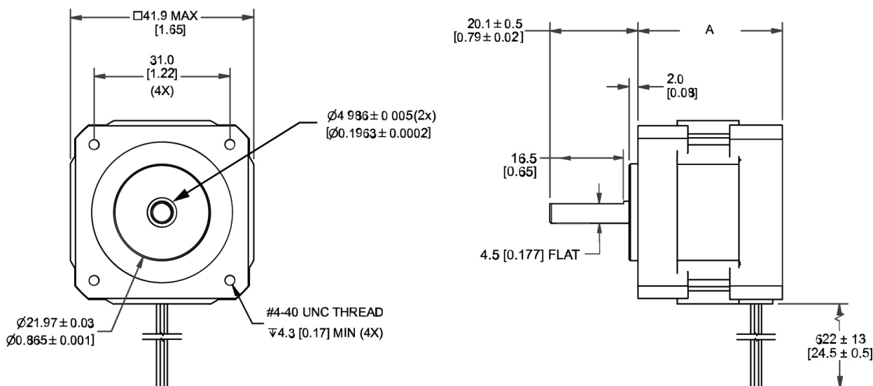
417-15-08 24VDC, 2.0 Amps/Phase, Bipolar, 1/2 Stepping
