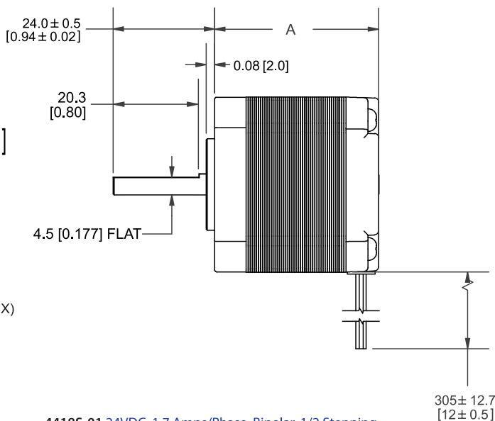
4418S-01 24VDC, 1.7 Amps/Phase, Bipolar, 1/2 Stepping
