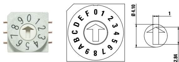
M0 Flush, Screw type "-&gt;"
