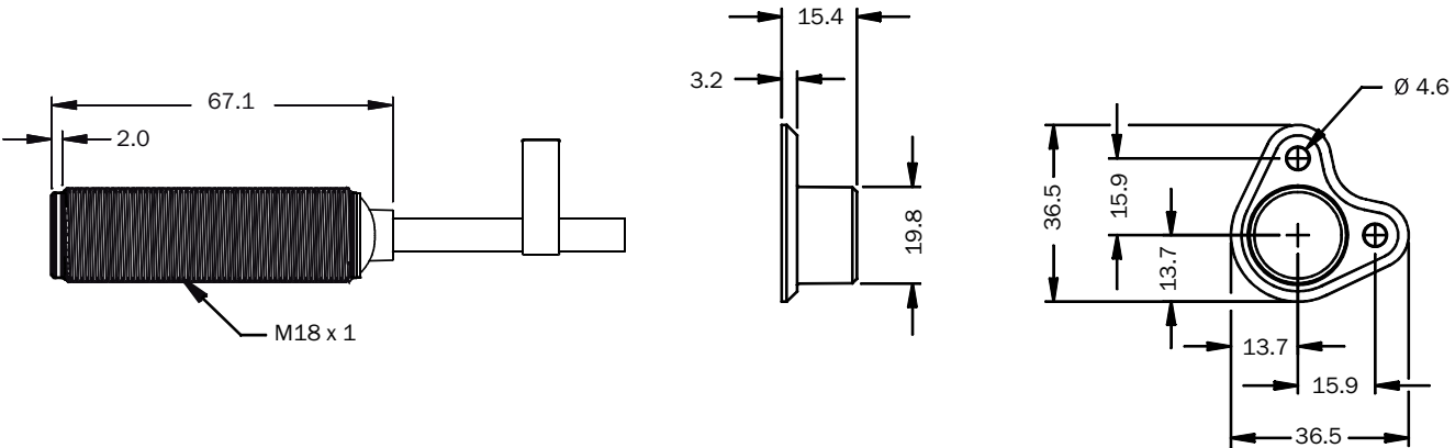
Dimensional drawing (Dimensions in mm (inch))
