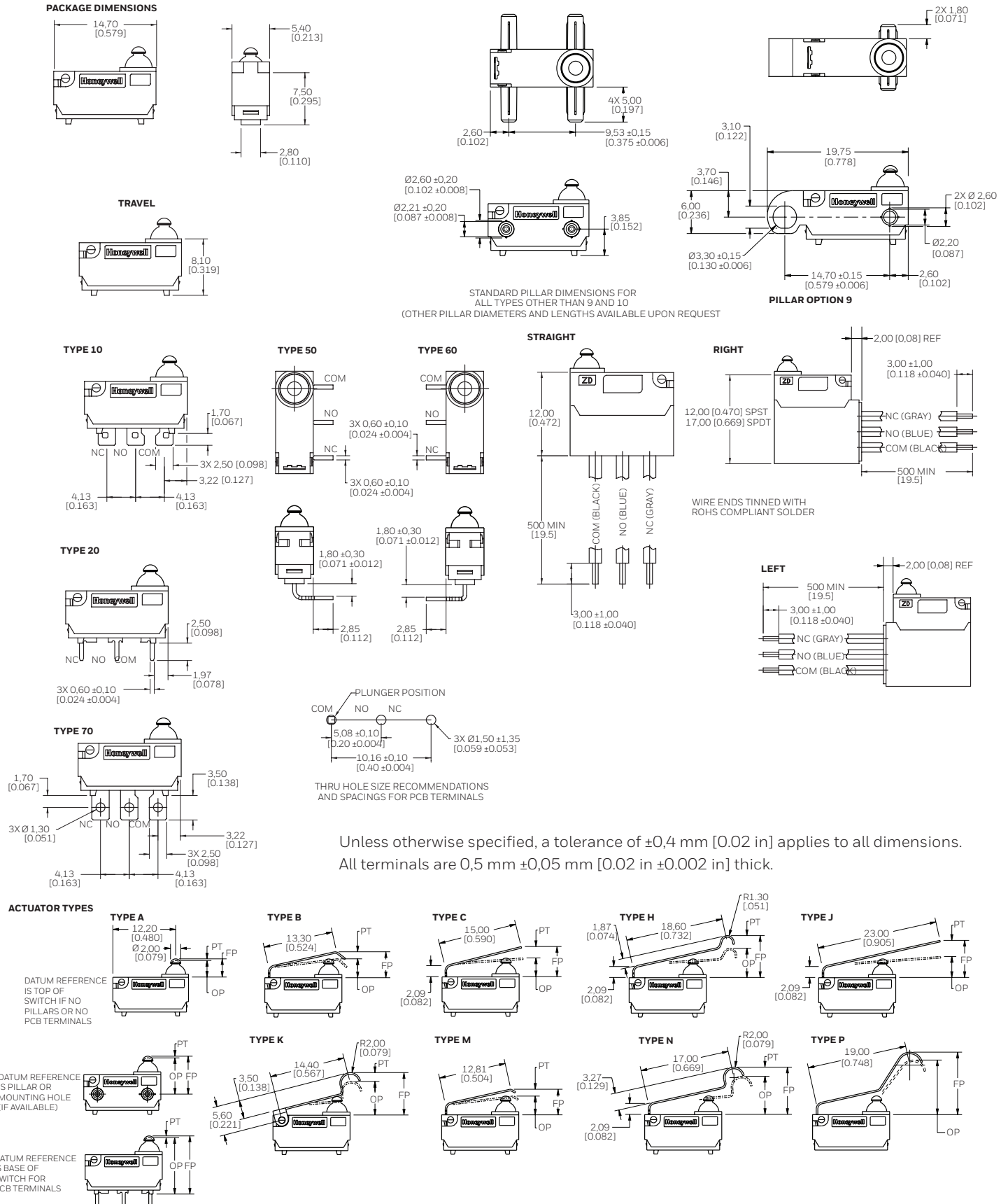
Figure 2. ZD Dimensions
