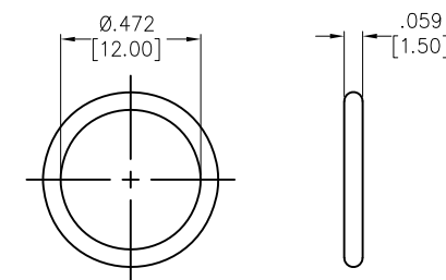
O-RING
