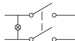
CIRCUIT DIAGRAM (DPST) ON-OFF
