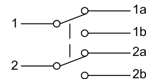
CIRCUIT DIAGRAM (DPDT) ON-ON
