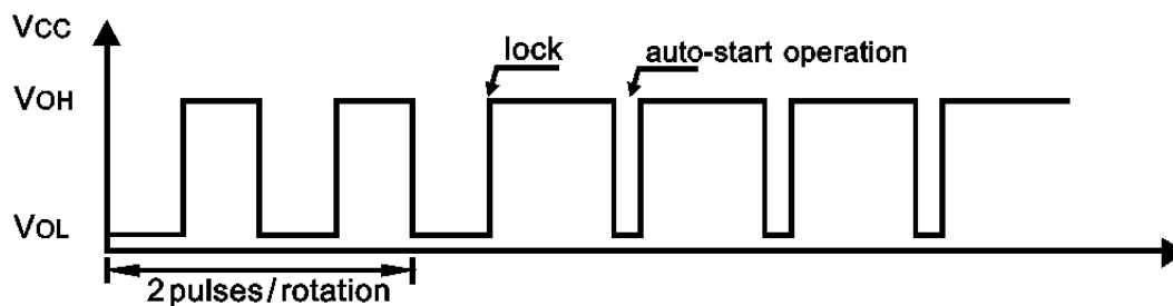
Output Waveform
