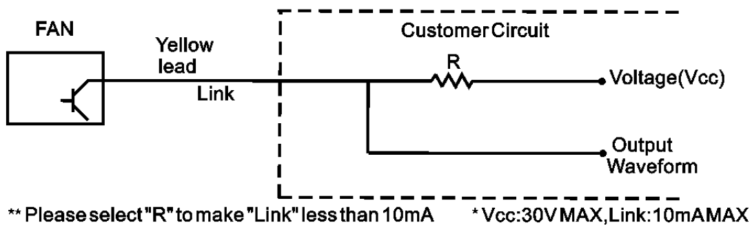
Output Waveform
