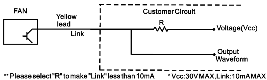
Output Waveform
