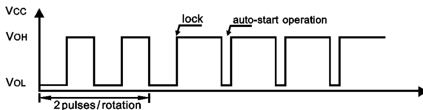
Output Waveform
