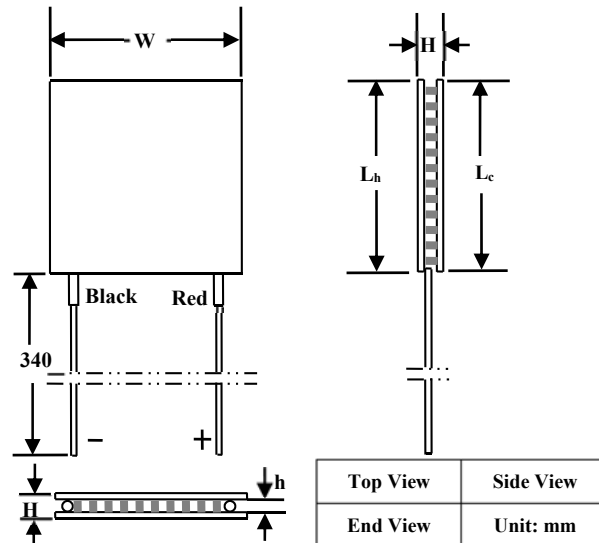
Figure 6. Mechanical Dimensions of ATE1-63-3.4A
