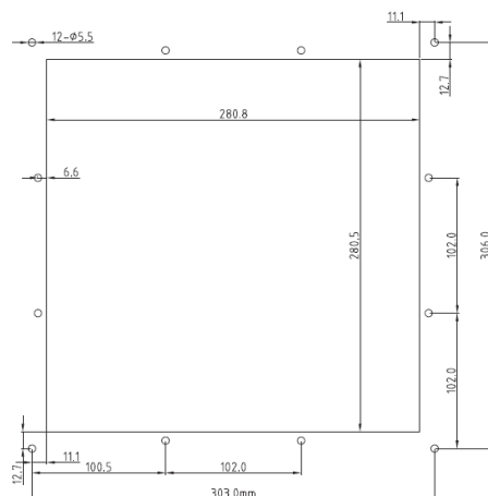
PANEL CUTOUT
