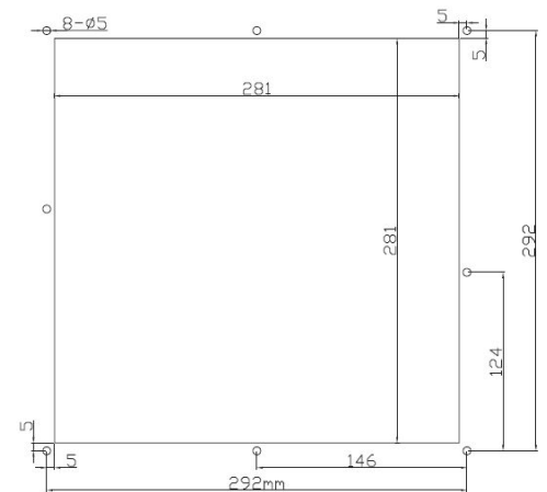
PANEL CUTOUT (REAR/INSIDE PERSPECTIVE)
