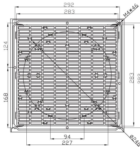
PANEL CUTOUT (REAR/INSIDE PERSPECTIVE)
