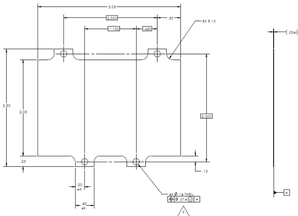
Figure 3-1. Mechanical Outline
