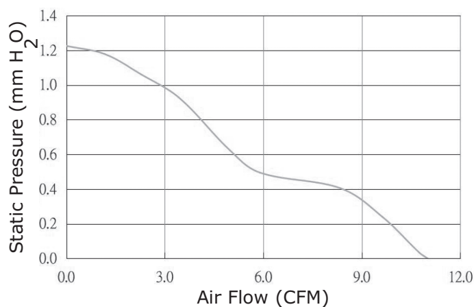
CFM-6015CF-245-332
