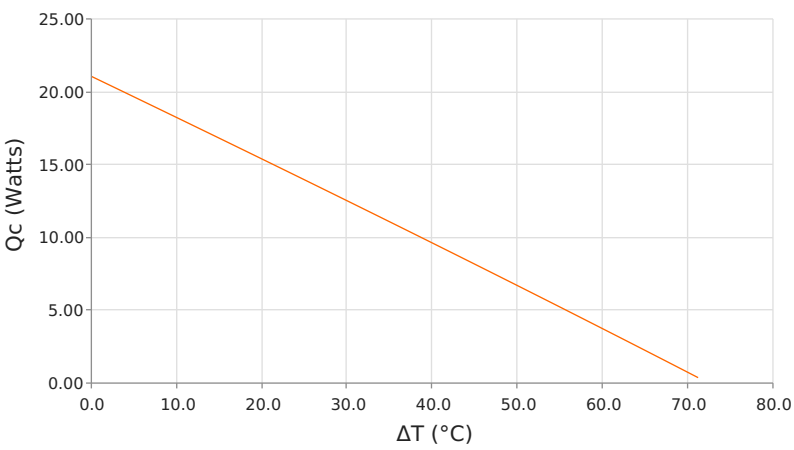
Heat Pumped at Cold Side ( Q_c ) T_{hot} = 35\text{ }^{\circ}\text{C} | I_{operating} = 2.2\text{ Amps}
