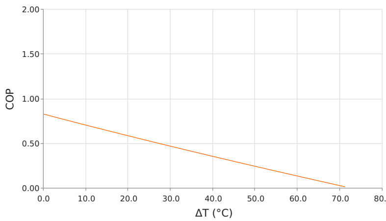
Coefficient of Performance (COP = Q_c/P_{in} ) T_{hot} = 35\text{ }^{\circ}\text{C} | I_{operating} = 2.2\text{ Amps}
