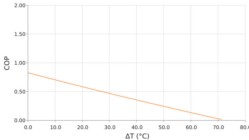
Coefficient of Performance (COP = Q_c/P_{in} ) T_{hot} = 35^\circ\text{C} | Operating = 6.2 Amps
