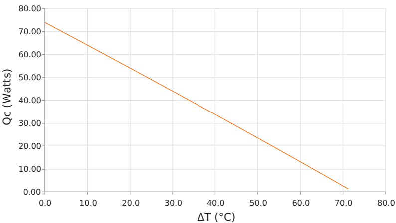
Heat Pumped at Cold Side ( Q_c ) T_{hot} = 35^\circ\text{C} | Operating = 6.2 Amps
