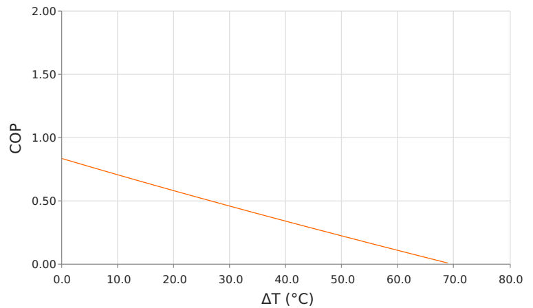
Coefficient of Performance (COP = Q_c/P_{in} ) T_{hot} = 27^\circ\text{C} | Current = 3.3 Amps
