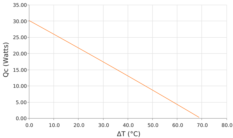
Heat Pumped at Cold Side ( Q_c ) T_{hot} = 27^\circ\text{C} | Current = 3.3 Amps
