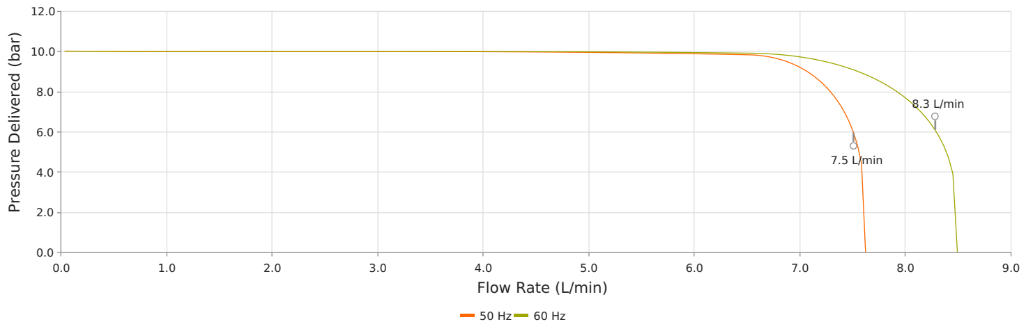
LA5000 - Pump Curve
