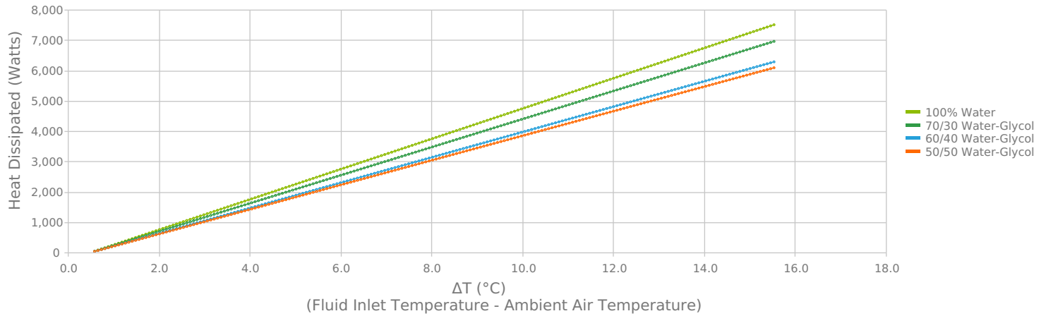
LA5000 Fluid Inlet/Outlet Temperature Difference ( \Delta T ) @ Nominal Flow 7.47 L/min
