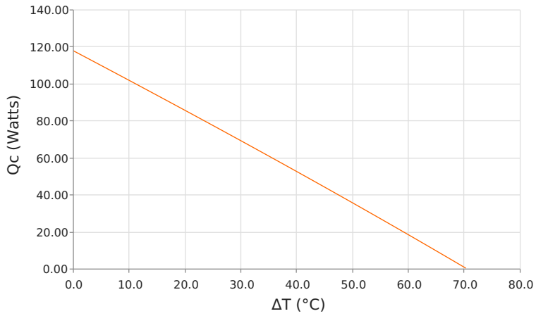
Heat Pumped at Cold Side ( Q_c ) T_{hot} = 27^\circ\text{C} | Current = 12.2 Amps
