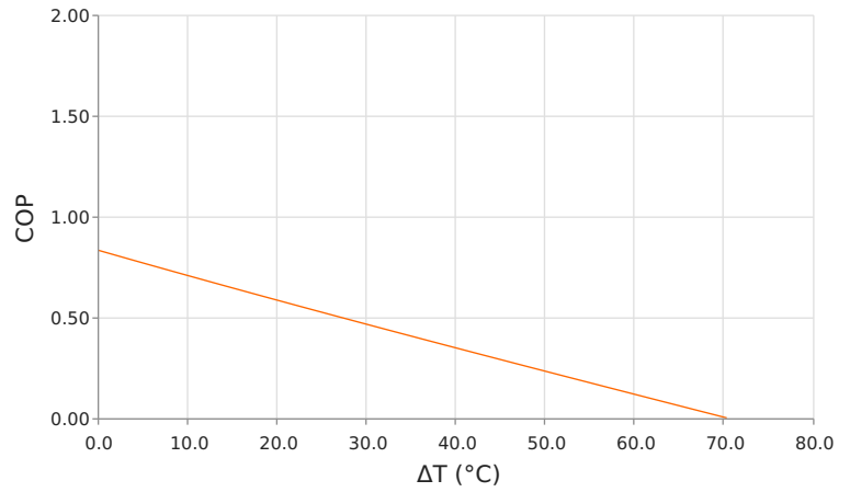
Coefficient of Performance (COP = Q_c/P_{in} ) T_{hot} = 27^\circ\text{C} | Current = 12.2 Amps
