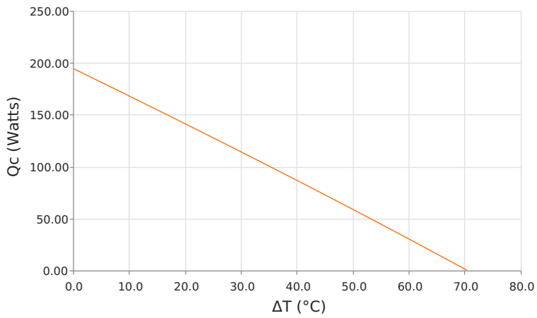
Heat Pumped at Cold Side ( Q_c ) T_{hot} = 27^\circ\text{C} | Current = 12.8 Amps
