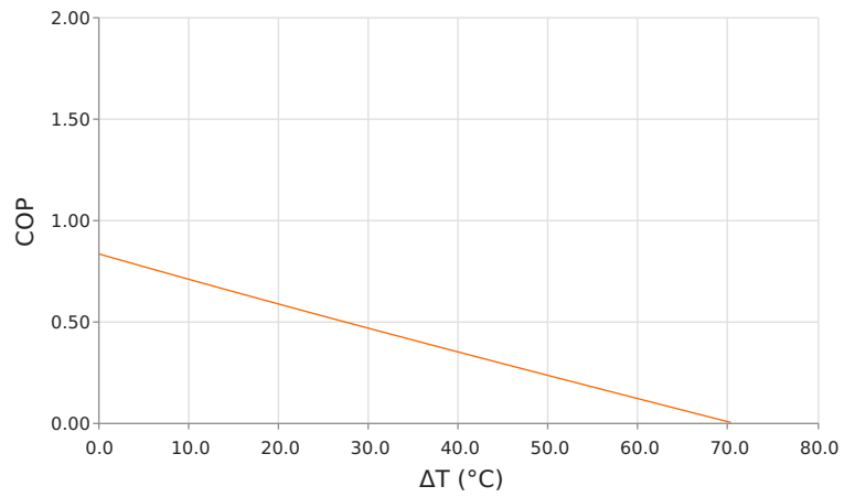
Coefficient of Performance (COP = Q_c/P_{in} ) T_{hot} = 27^\circ\text{C} | Current = 12.8 Amps
