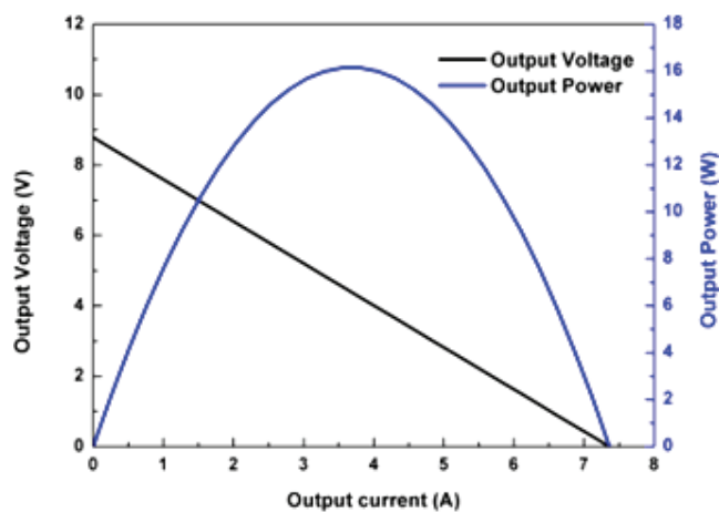
Output Voltage/Power Vs. Output Current (Th=300°C, Tc=30°C)
