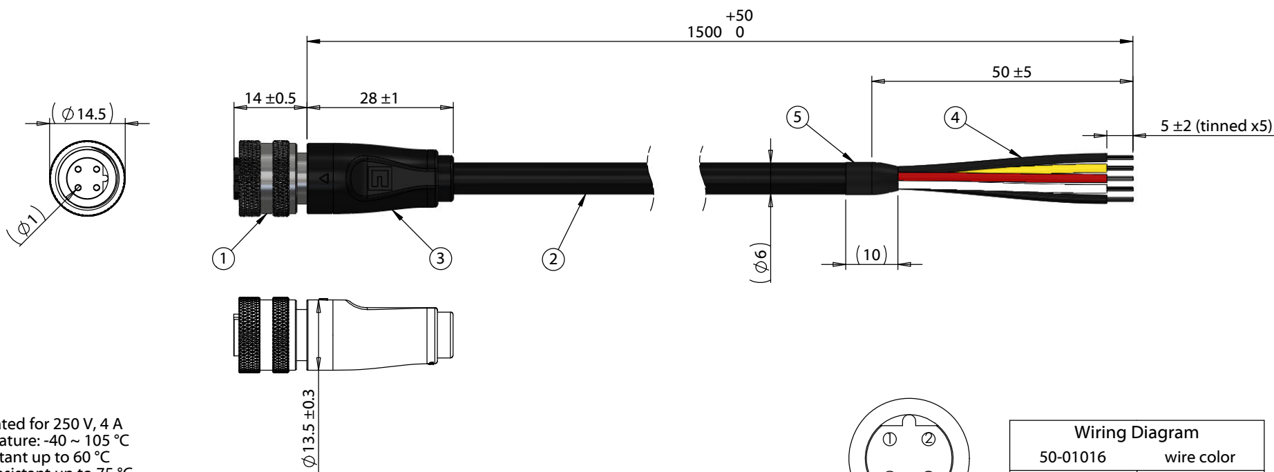
Front View Not to Scale
