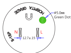
(NEMA 5-15P, Hospital Grade) (Dimensions of Plug Face)
