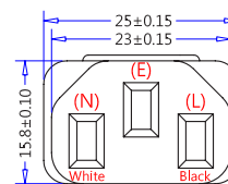
(IEC 60320, C13, 13A 125V~) (Dimensions of Connector Face)
