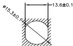
Panel hole size
