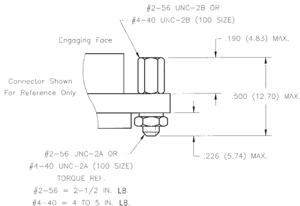
Removable Jackpost
