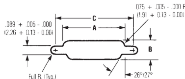
Rear Mounting
