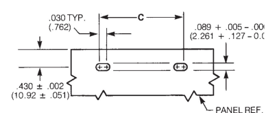
Figure 3. Edgeboard Mounting
