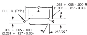
Figure 2. Rear Mounting
