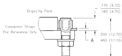
Jackpost Bushing
