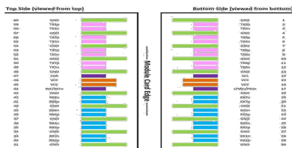
Electrical Pin-out Details for OSFP
