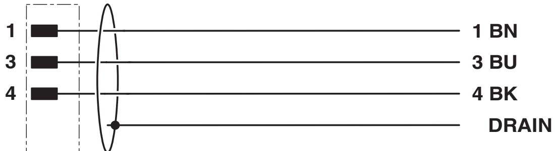
Circuit diagram
