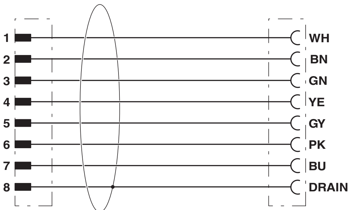
Circuit diagram
