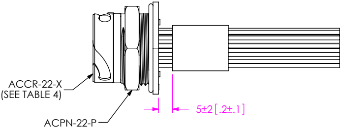
IN-PROCESS 6 THREAD ACPN-22-P ONTO ACPFS-22-P-X STRETCH ACCR-22-X OVER ACPFS-22-P-X UNTIL IT SEATS IN GROOVE. ACTIVATE HEAT SHRINK TUBING.
