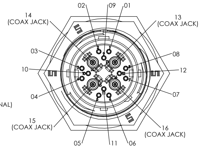
-06: 16 POS COMBO 4 X COAX JACK 12 X 1.0 SOCKETS
