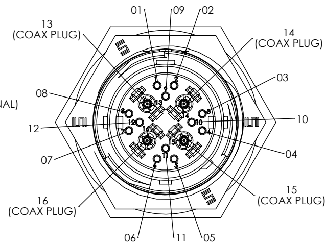
-06: 16 POS COMBO (4 X COAX PLUGS) (12 X 1.0 Ø TERMINALS)
