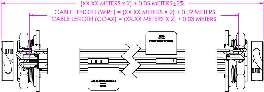
IN-PROCESS 7 (-BC OPTION ONLY) BUILD DOUBLE-ENDED INITIALLY FOR E-TEST, APPLY LABEL-ET & HDRL-11 TO BOTH ENDS, AND CUT CABLE IN HALF
