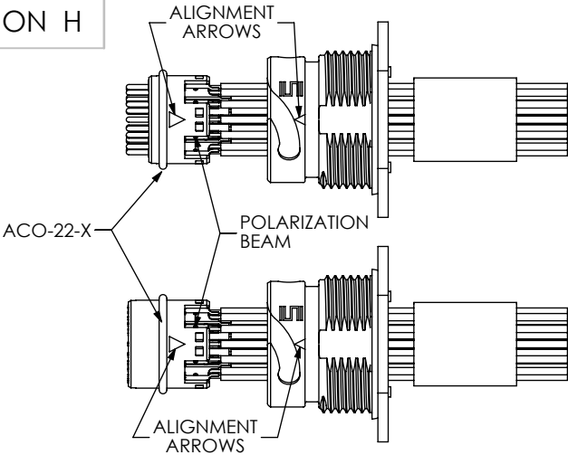
IN-PROCESS 3 PUSH ACO-22-1 ORING ONTO SUB-ACTHB-22-X-X OR SUB-ACSHB-22-X-X SUB-ASSEMBLIES
