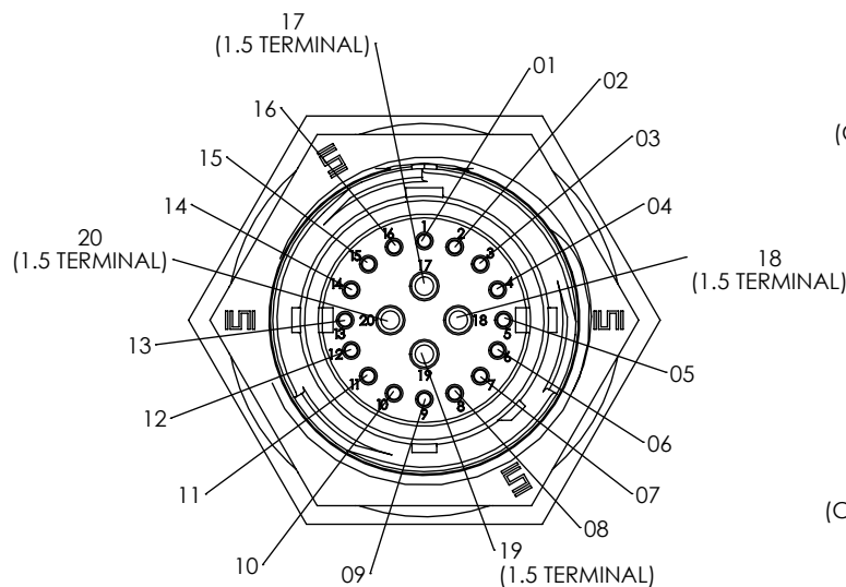
-05: 20 POS COMBO (4X Ø 1.5 TERMINALS) (16 X Ø 1.0 TERMINALS)
