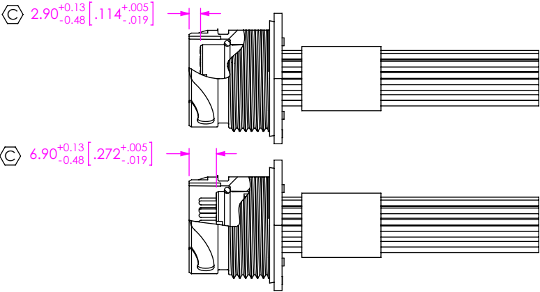
IN-PROCESS 4 WHILE MAKING SURE ALIGNMENT ARROWS LINE UP TO AID POLARIZATION BEAM ENGAGEMENT, INSERT SUB-ACXHB-22-X SUB-ASSEMBLY INTO ACPFS-22-P-X PANEL SHELL UNTIL SNAP LOCKS ENGAGE
