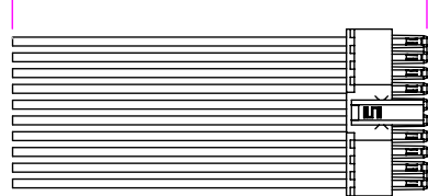
-02: 20 POS (MMSD-10-24-L-XX.XX-S-K)
