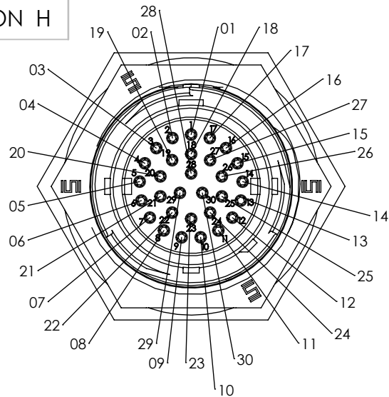
-01: 30 POS (Ø 1.0 SOCKETS)
