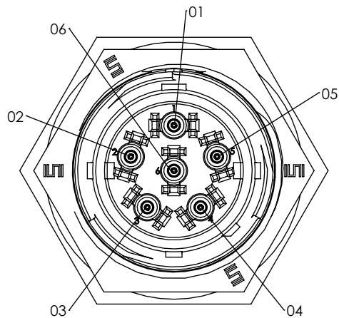
-04: 6 POS (COAX JACK)
