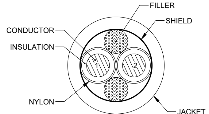
CROSS-SECTIONAL VIEW
