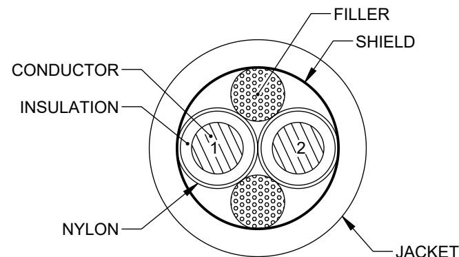
CROSS-SECTIONAL VIEW
