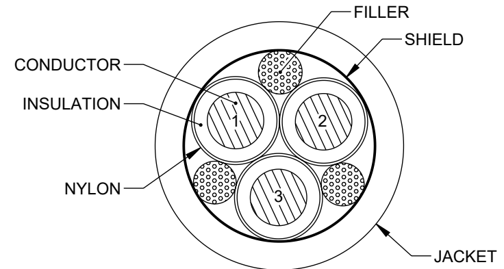
CROSS-SECTIONAL VIEW
