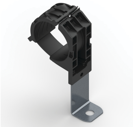
Ratchet P-Clamp, 1.38 - 2.01" Bundle Dia, 90° Long, 0.41" Hole Dia, PA666V0/SS304, Black, 140/ctn
