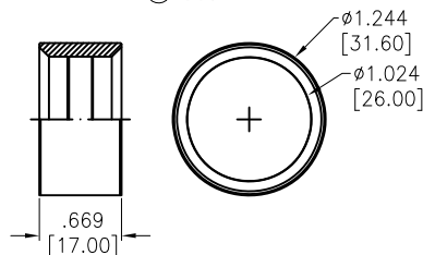
Ⓓ Seal
