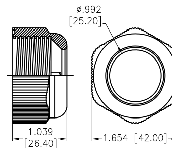
Ⓔ Sealing Nut
