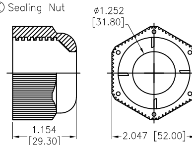
Ⓔ Sealing Nut
